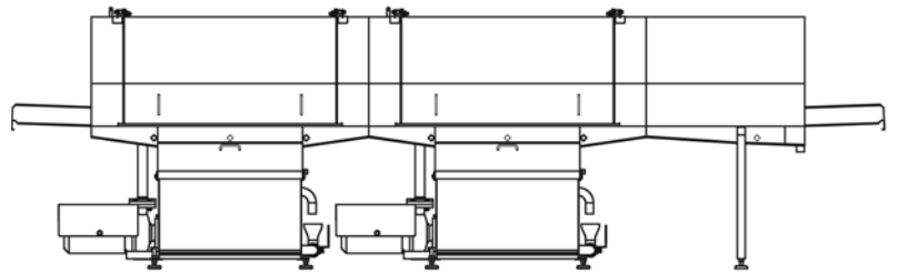
Modular multi-zone tunnel washing machines, module length 1750 mm with a transport width of maximum 60 cm.
