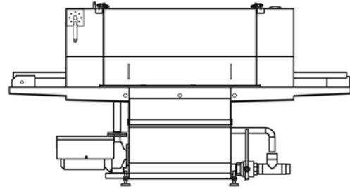
Dual-zone tunnel washing machine with a transport width of maximum 40 and 60 cm.
